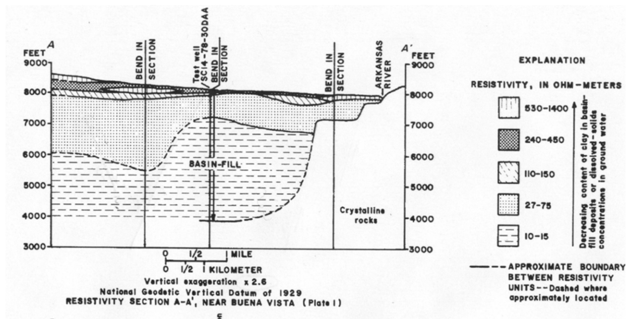
Figure 3-1. East-west electrical resistivity cross-section across the Upper Arkansas Valley about 3 miles south of Buena Vista. From Crouch and others, 1984, after Zohdy and others, 1971.
