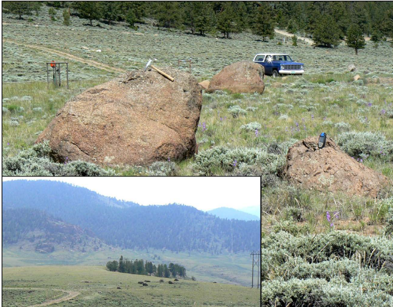
Fig. 6-3. Close-up of ice-rafted boulders that mark the shoreline of Three Glaciers Lake at 9834 ft elevation (2861 m). Inset at lower left shows the geomorphic setting of the boulder cluster, which can be seen in lower right center.
