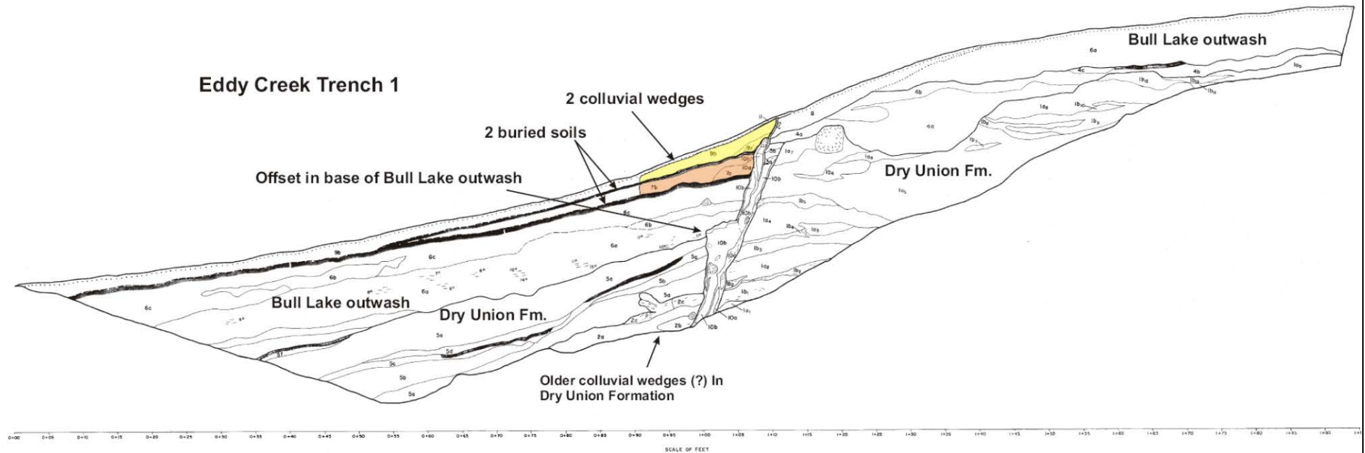
Figure 1-6. Trench ET-1 exposed two major units: 1) Dry Union Formation alluvial-fan and colluvial materials (units 1-5 on trench log), overlain by 2) Bull Lake outwash (unit 6 on trench log). The fault (unit 10) is an anastomosing shear zone up to a meter wide, dipping 70° east. Multiple faulting episodes in the Dry Union Formation are shown by (1) a truncated fault zone within the Dry Union (between units 1 and 3), and (2) stone lines and buried soils in colluvial unit 5 of Dry Union age on the downdropped side of the fault. These displacements do not contribute to the present scarp height. One mapped fault splay is truncated by the Bull Lake outwash, suggesting an event during Bull Lake outwash deposition.
